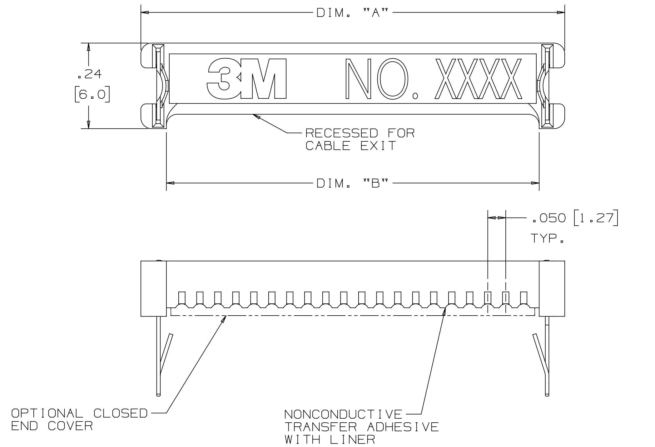
COVER ASSEMBLY
