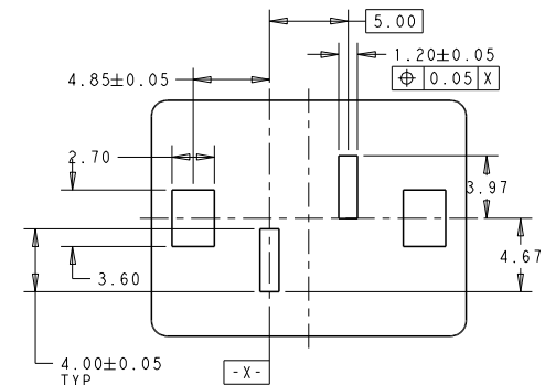
LAYOUT FOR 1-2834235-2
