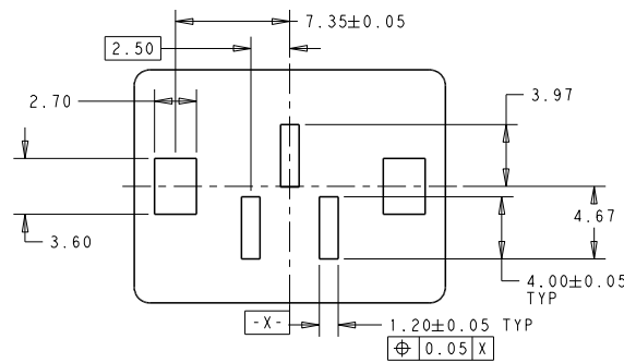
LAYOUT FOR 1-2834235-1
