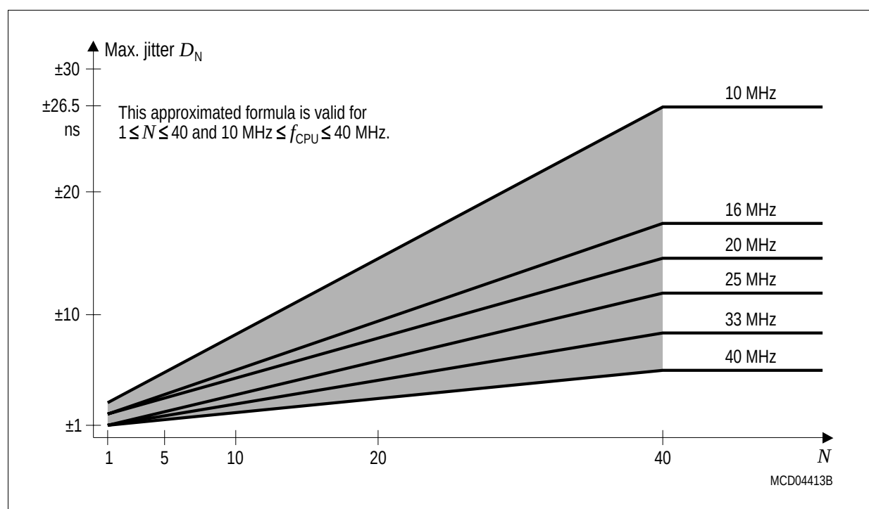
Figure 12 Approximated Maximum Accumulated PLL Jitter
