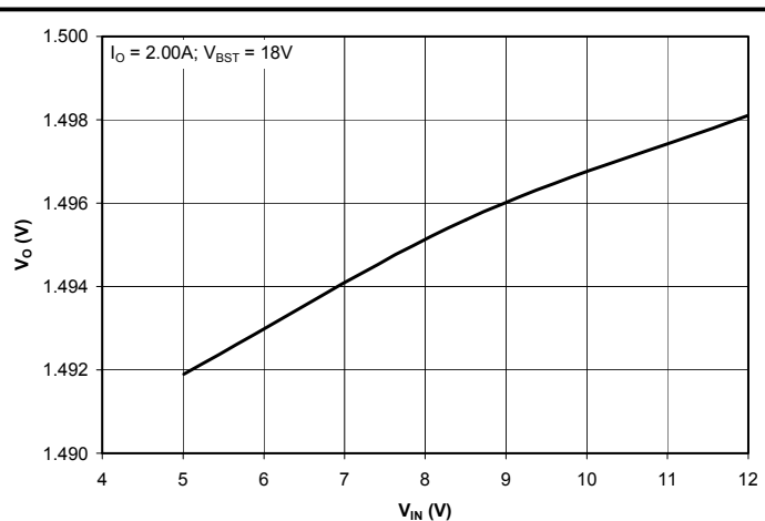
Typical Line Regulation
