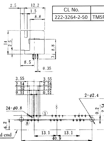
PCB mounting hole layout (Connector mounting side)
