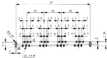
TM2REA-2424 (50)
