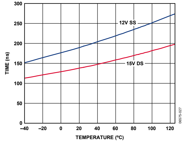
Figure 14. t_{\text{TRANSITION}} Time vs. Temperature
