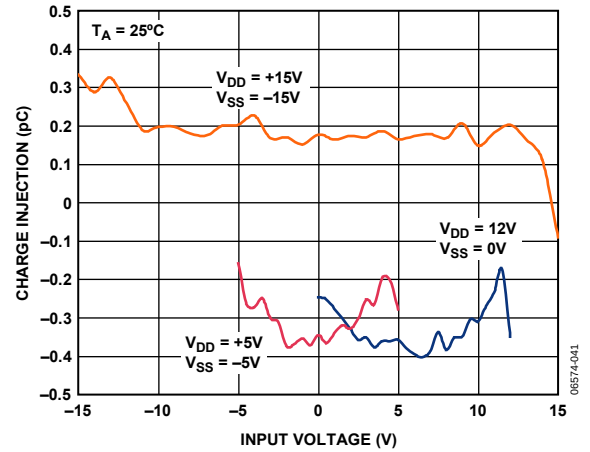
Figure 13. Charge Injection vs. Input Voltage
