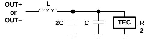
Figure 11. LC Half-Circuit Equivalent
