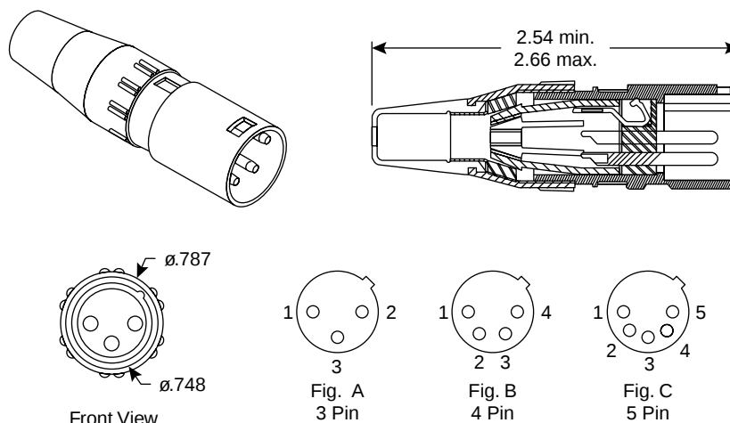
Dimensions (In.)
