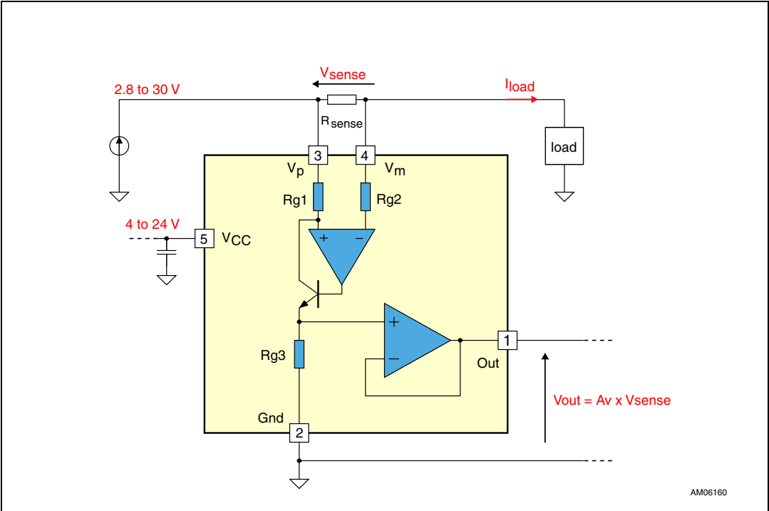
Figure 1. Application schematics
