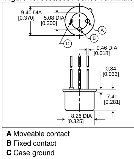
Figure 18. 3600/3601 Series Terminals
