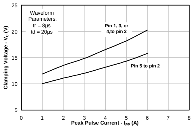
TLP Characteristic (Pin 1, 3, or 4 to GND)
