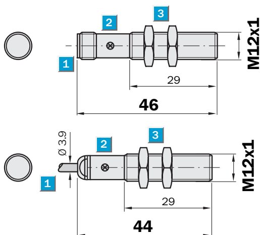
Dimensional drawing
