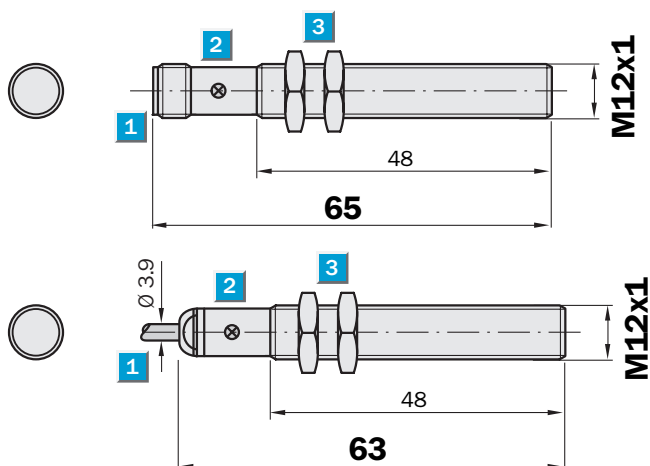
Dimensional drawing
