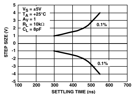
FIGURE 24. STEP SIZE vs SETTLE TIME
