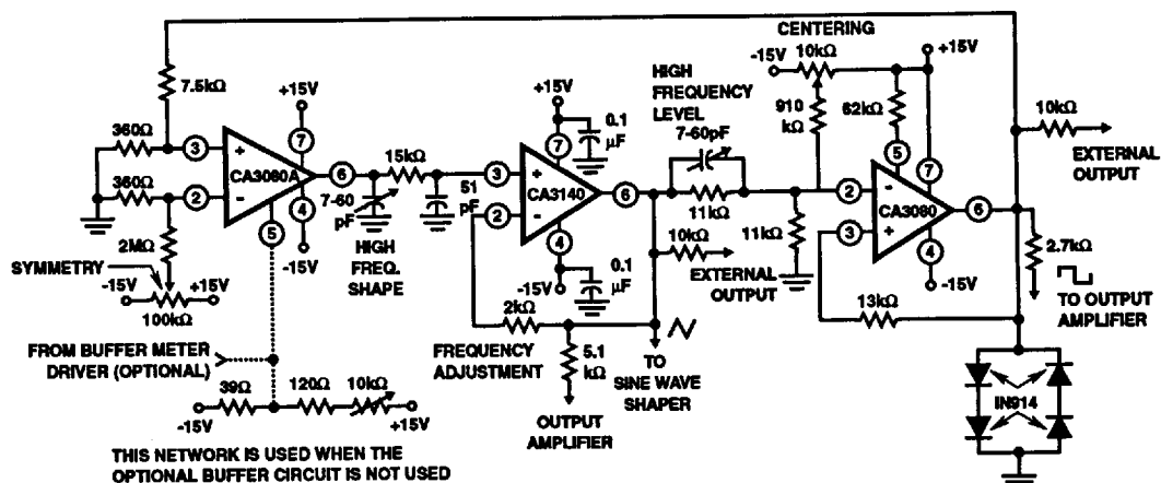
(A) CIRCUIT
