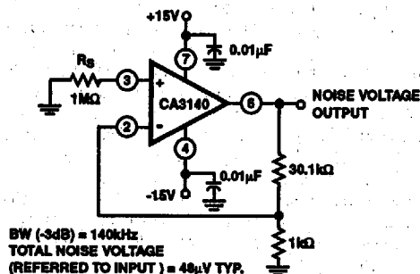
FIGURE 35. TEST CIRCUIT AMPLIFIER (30dB GAIN) USED FOR WIDEBAND NOISE MEASUREMENT
