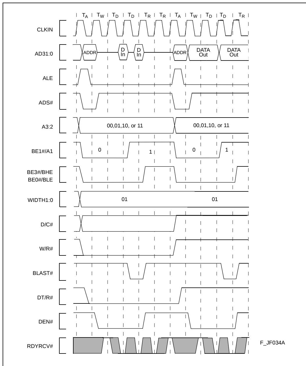
Figure 46. Burst Read and Write Transactions With 1, 0 Wait States and Extra Tr State on Read, 16-Bit Bus
