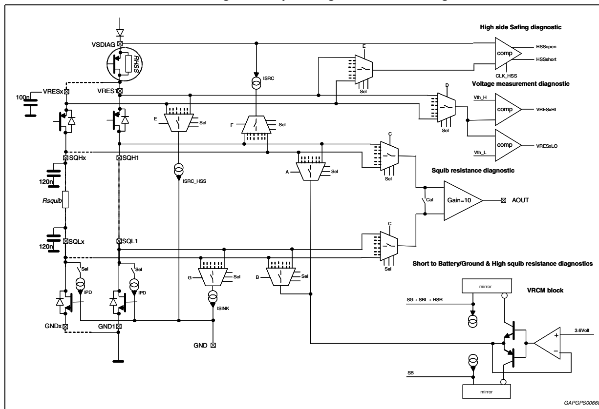
Figure 9. Squib diagnostics block diagram
