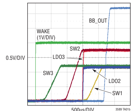
Start-Up Sequence
