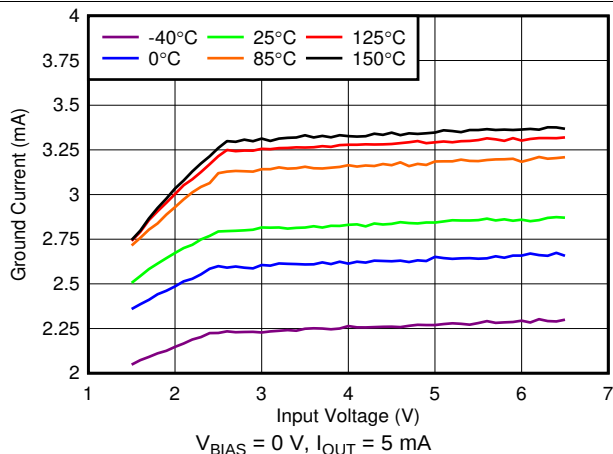
Figure 27. Quiescent Current vs Input Voltage
