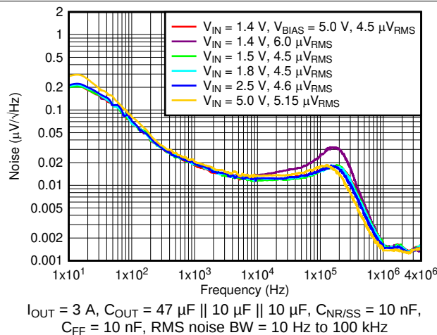
Figure 11. Output Noise vs Frequency and V_{IN}
