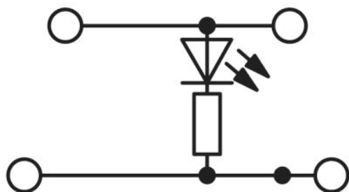
Circuit diagram
