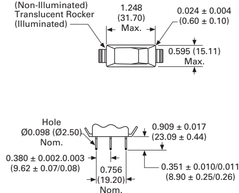
Code "B" Alternative Solder Lug Only
