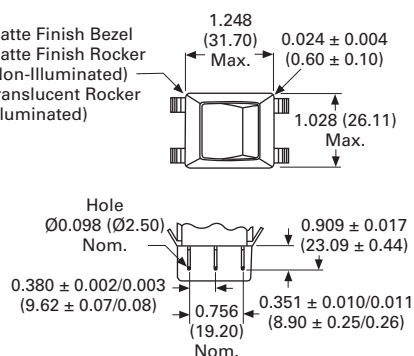
Code "B" Alternative Solder Lug Only
