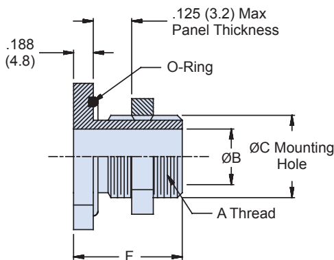
Bulkhead Adapters 710-100/101/372
