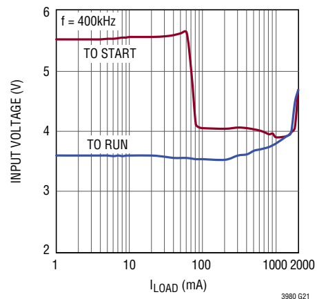
Minimum Input Voltage, V_{OUT} = 3.3\text{V}
