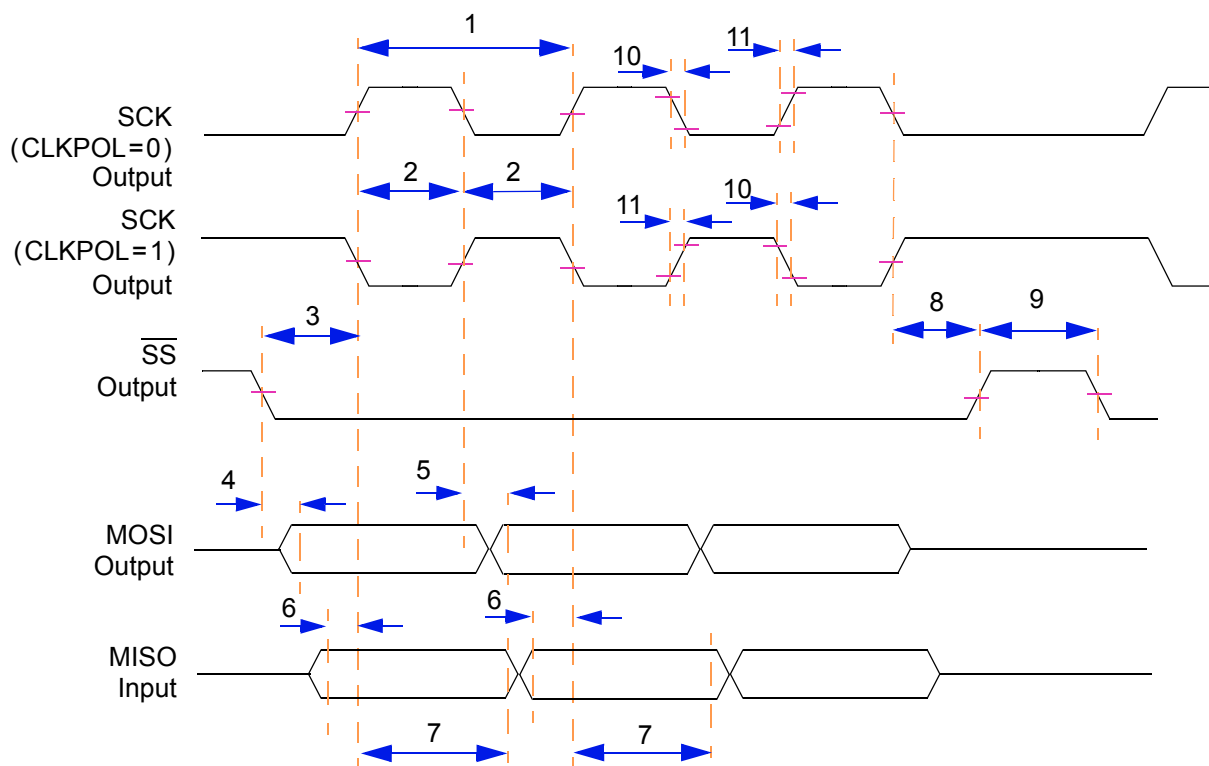
Figure 42. Timing Diagram — SPI Master Mode, Format 0 (CPHA = 0)
