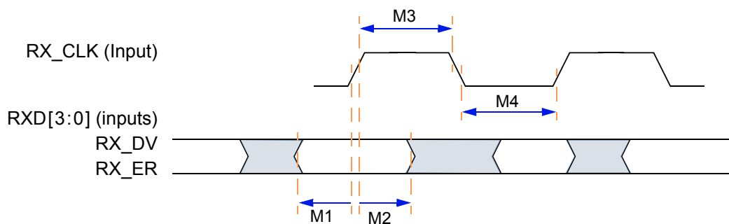
Figure 28. Ethernet Timing Diagram—MII Rx Signal
