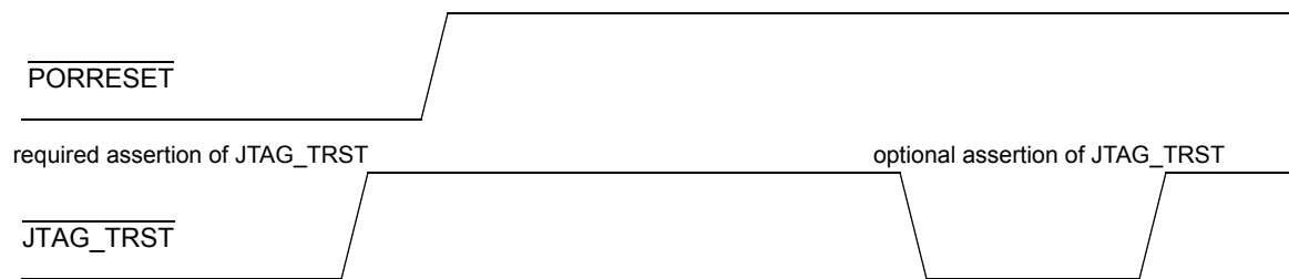
Figure 54. \overline{\text{PORRESET}} vs. \text{JTAG\_TRST}
