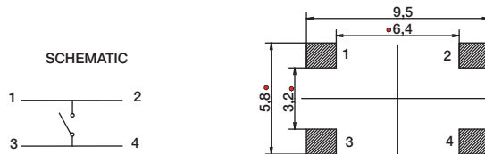
PCB LAYOUT
