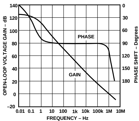
Figure 19. Open-Loop Gain and Phase vs. Frequency
