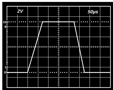
Figure 23b. Unity Gain Inverter Large Signal Pulse Response, C_L = 1,000 \text{ pF}
