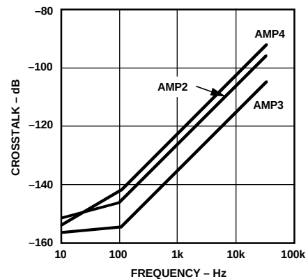
Figure 2b. Crosstalk vs. Frequency
