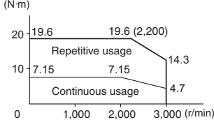
R88M-G1K520T (1.5 kW)
