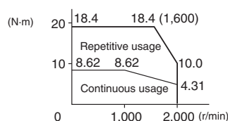
R88M-G90010T (900 W)
