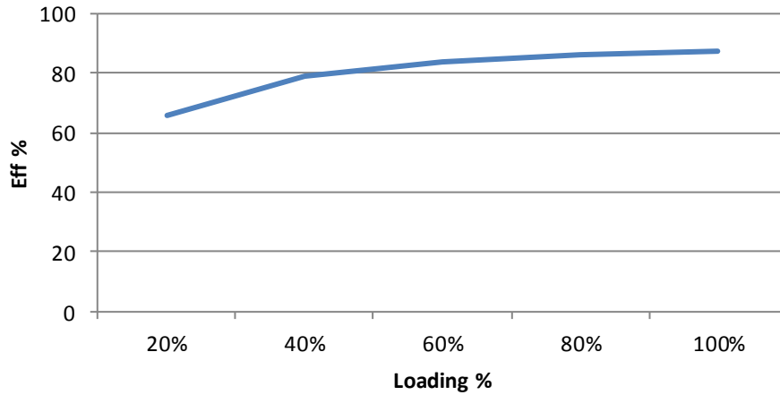
AM1D-0515S-RZ Efficiency vs. Loading
