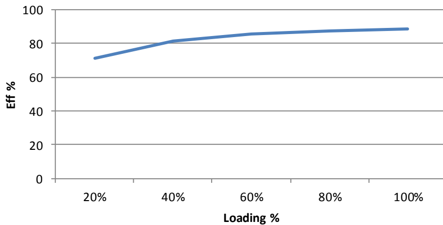
AM1D-1209S-RZ Efficiency vs. Loading
