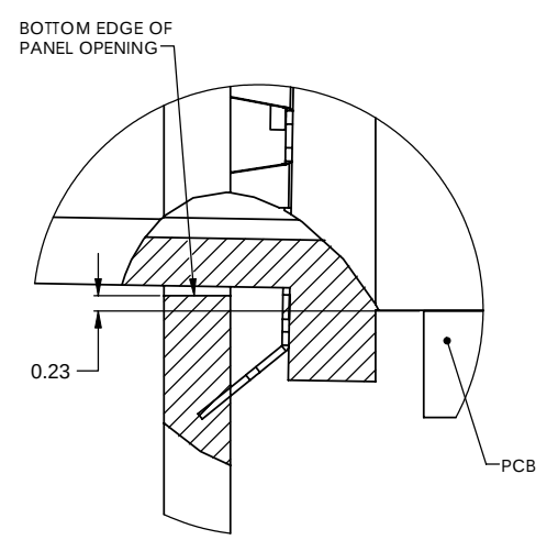
DETAIL J SCALE 16 : 1
