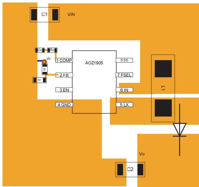
(a) MSOP-8
