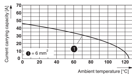
Derating diagram (6 modules in HC-B 24 housing)
