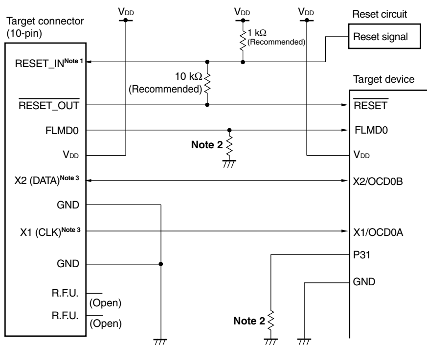
Figure 27-1. Connection Example of QB-78K0MINI or QB-MINI2 and \mu PD78F0527D (When OCD0A/X1 and OCD0B/X2 Are Used)
