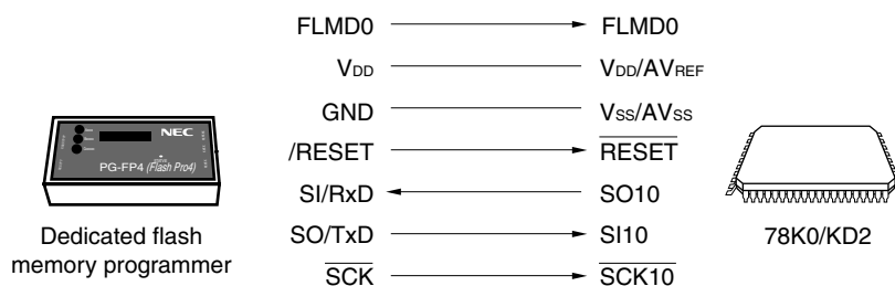
Figure 26-6. Communication with Dedicated Flash Memory Programmer (CSI10)
