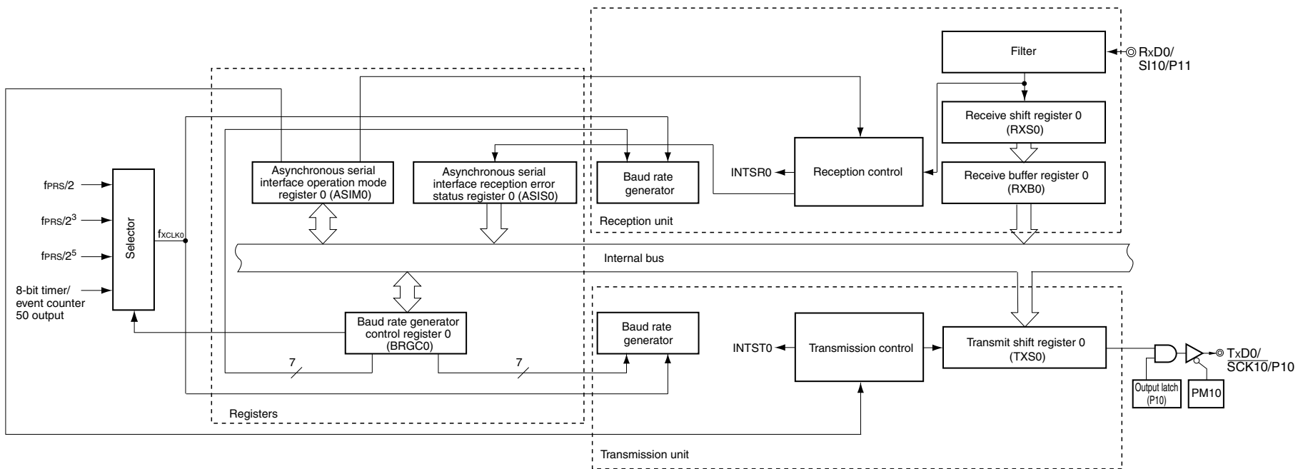
<R> Figure 14-1. Block Diagram of Serial Interface UART0
