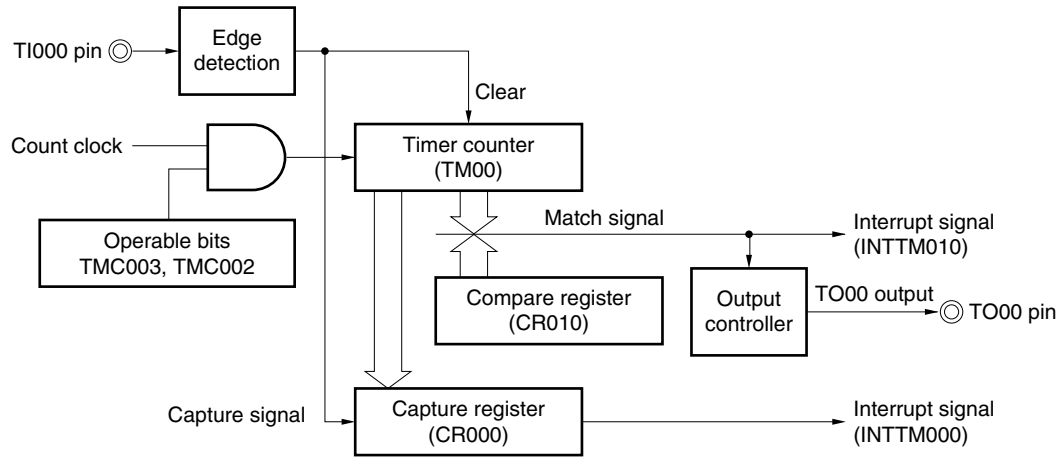
Figure 7-26. Block Diagram of Clear & Start Mode Entered by TI000 Pin Valid Edge Input (CR000: Capture Register, CR010: Compare Register)
