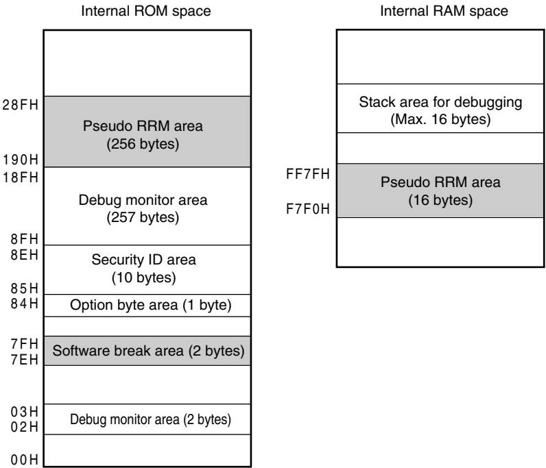
Figure 27-4. Reserved Area Used by QB-78K0MINI and QB-MINI2
