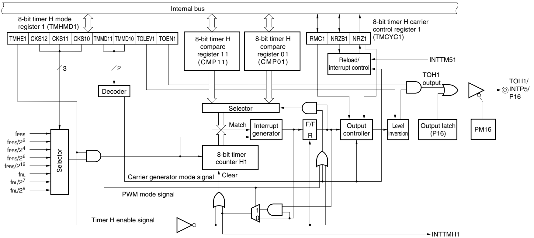
&lt;R&gt; Figure 9-2. Block Diagram of 8-Bit Timer H1
