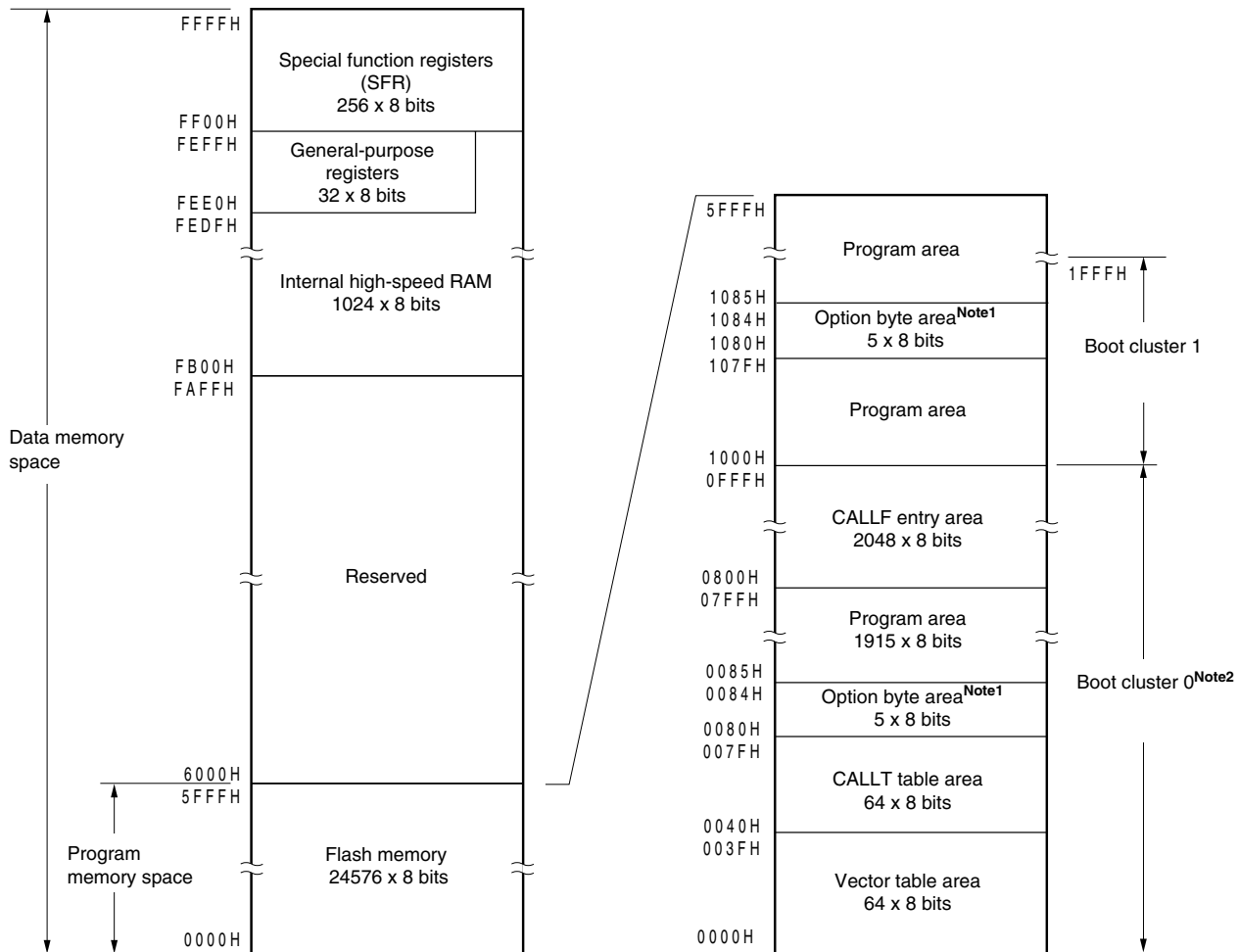
Figure 3-2. Memory Map ( \mu PD78F0522)
