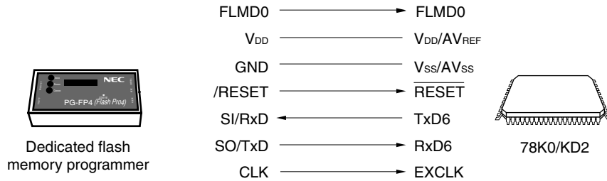
Figure 26-7. Communication with Dedicated Flash Memory Programmer (UART6)
