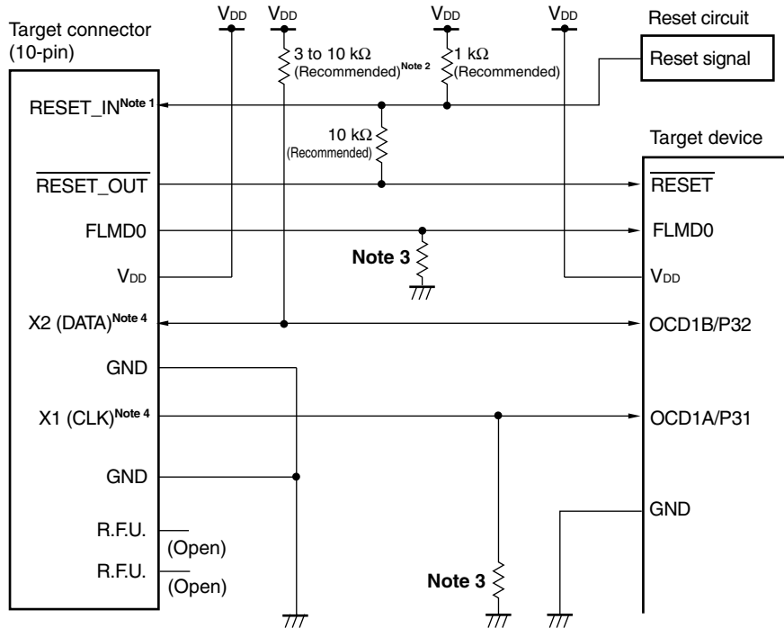
Figure 27-2. Connection Example of QB-78K0MINI and \mu PD78F0527D (When OCD1A/P31 and OCD1B/P32 Are Used)
