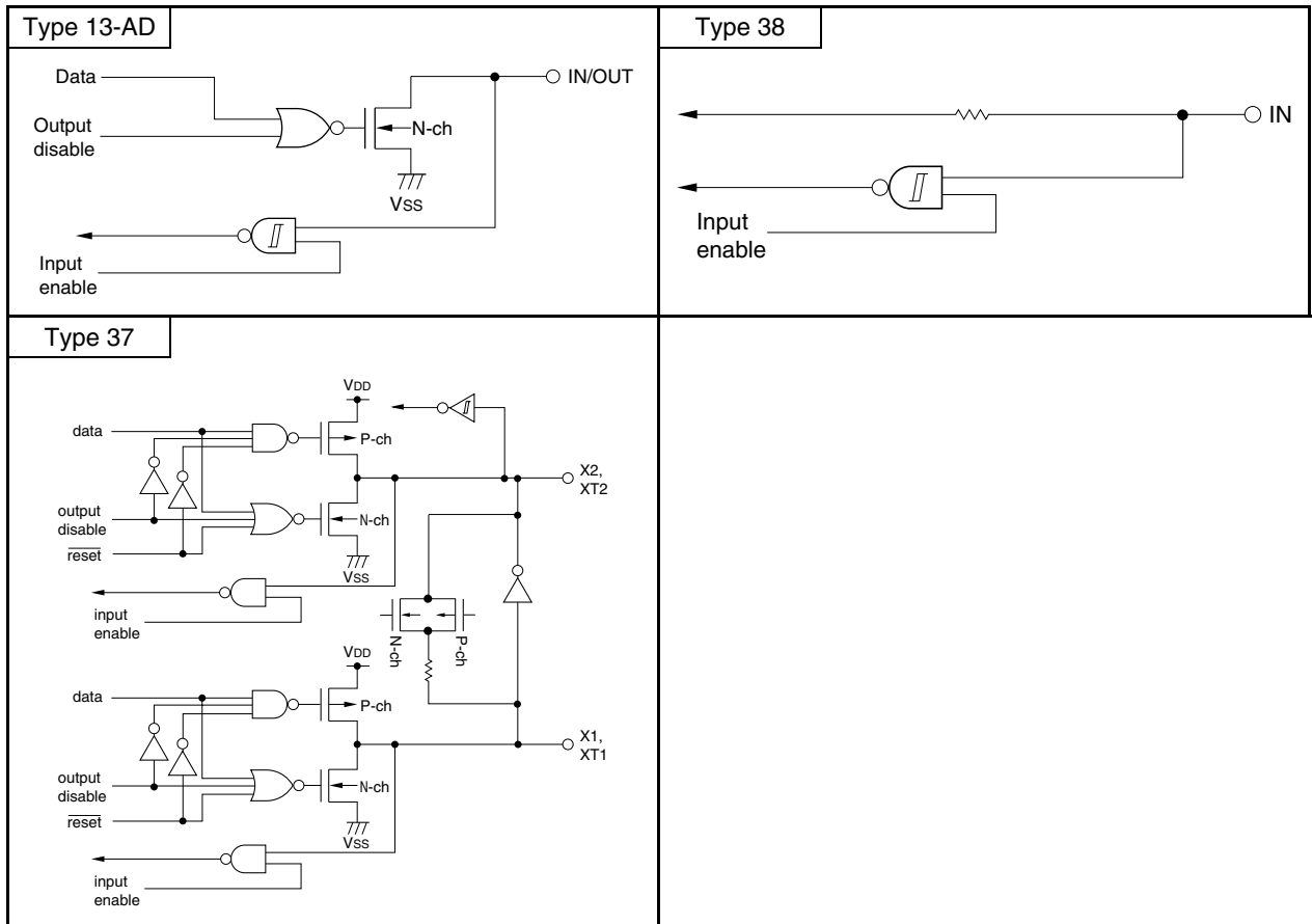
Figure 2-1. Pin I/O Circuit List (2/2)
