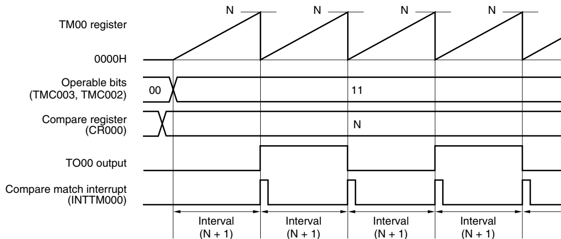
<R> Figure 7-16. Basic Timing Example of Square Wave Output Operation
