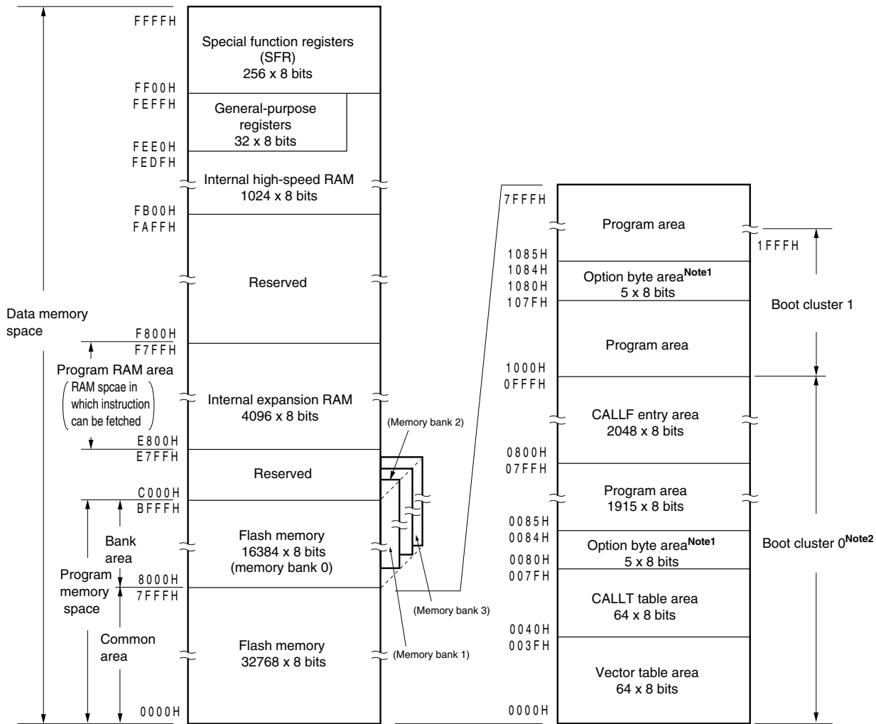
Figure 3-6. Memory Map (μPD78F0526)
