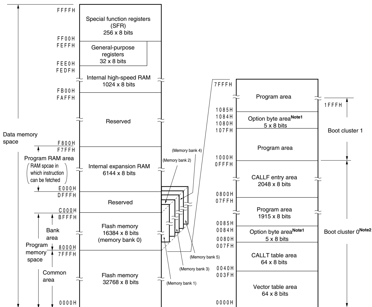
Figure 3-7. Memory Map ( \mu PD78F0527)
