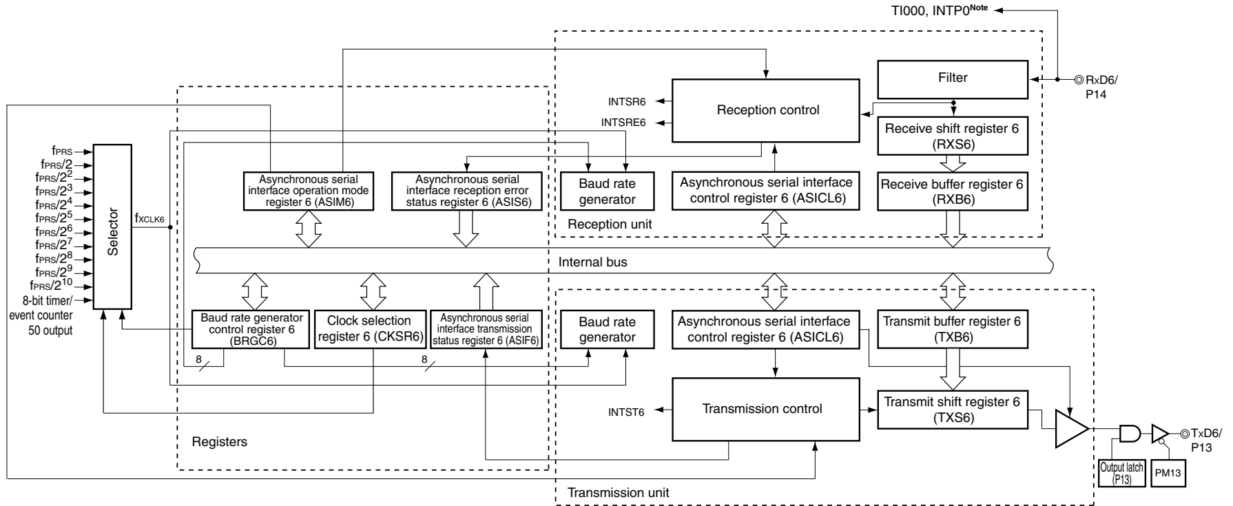
&lt;R&gt;Figure 15-4. Block Diagram of Serial Interface UART6
