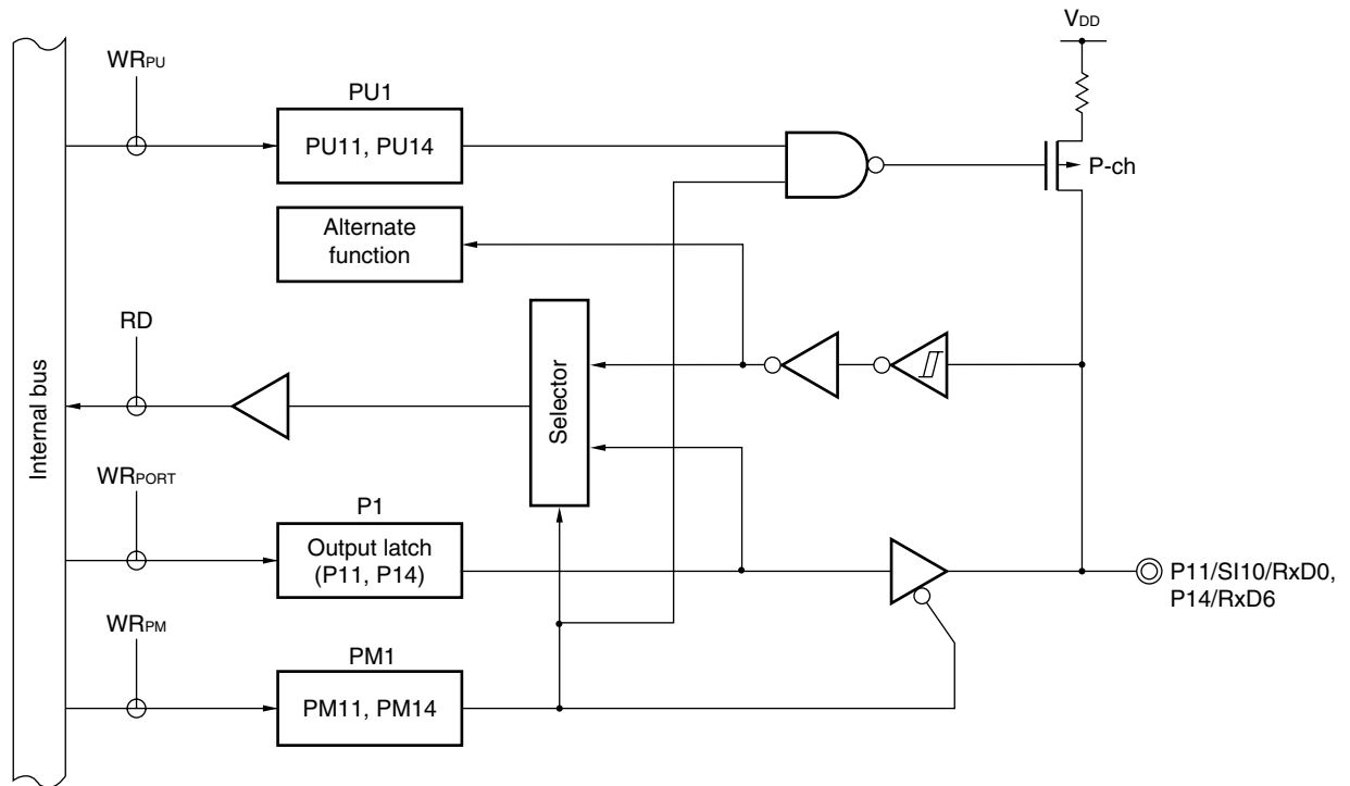
Figure 5-6. Block Diagram of P11 and P14
