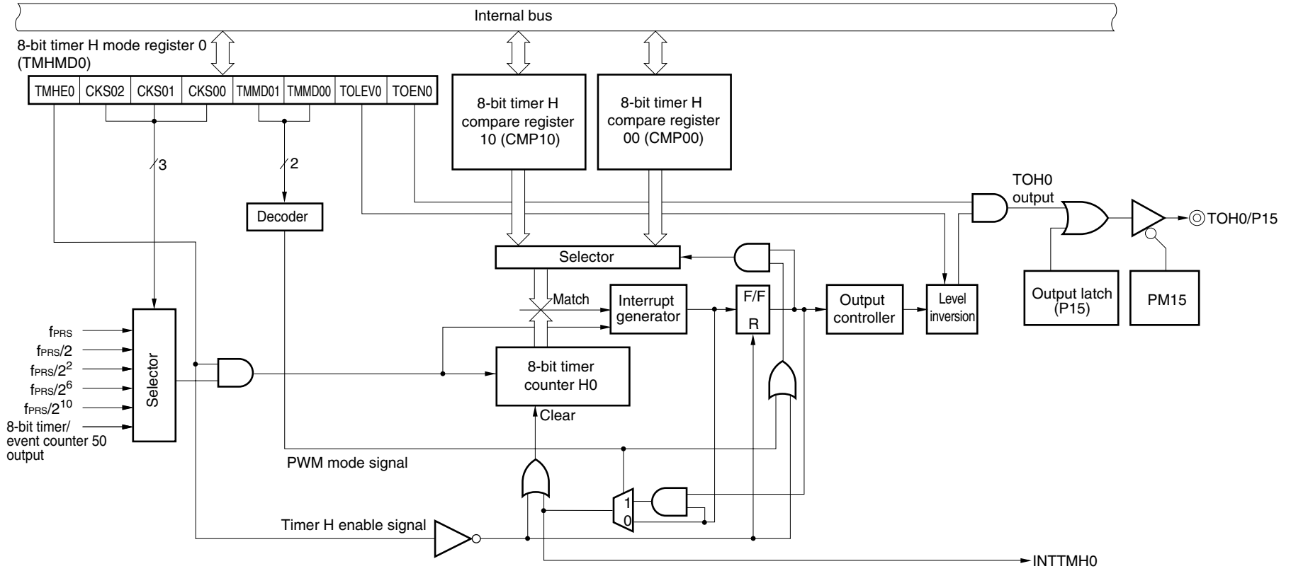
<R> Figure 9-1. Block Diagram of 8-Bit Timer H0
