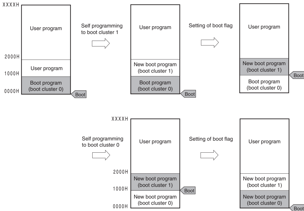
<R> Figure 26-17. Boot Swap Function
