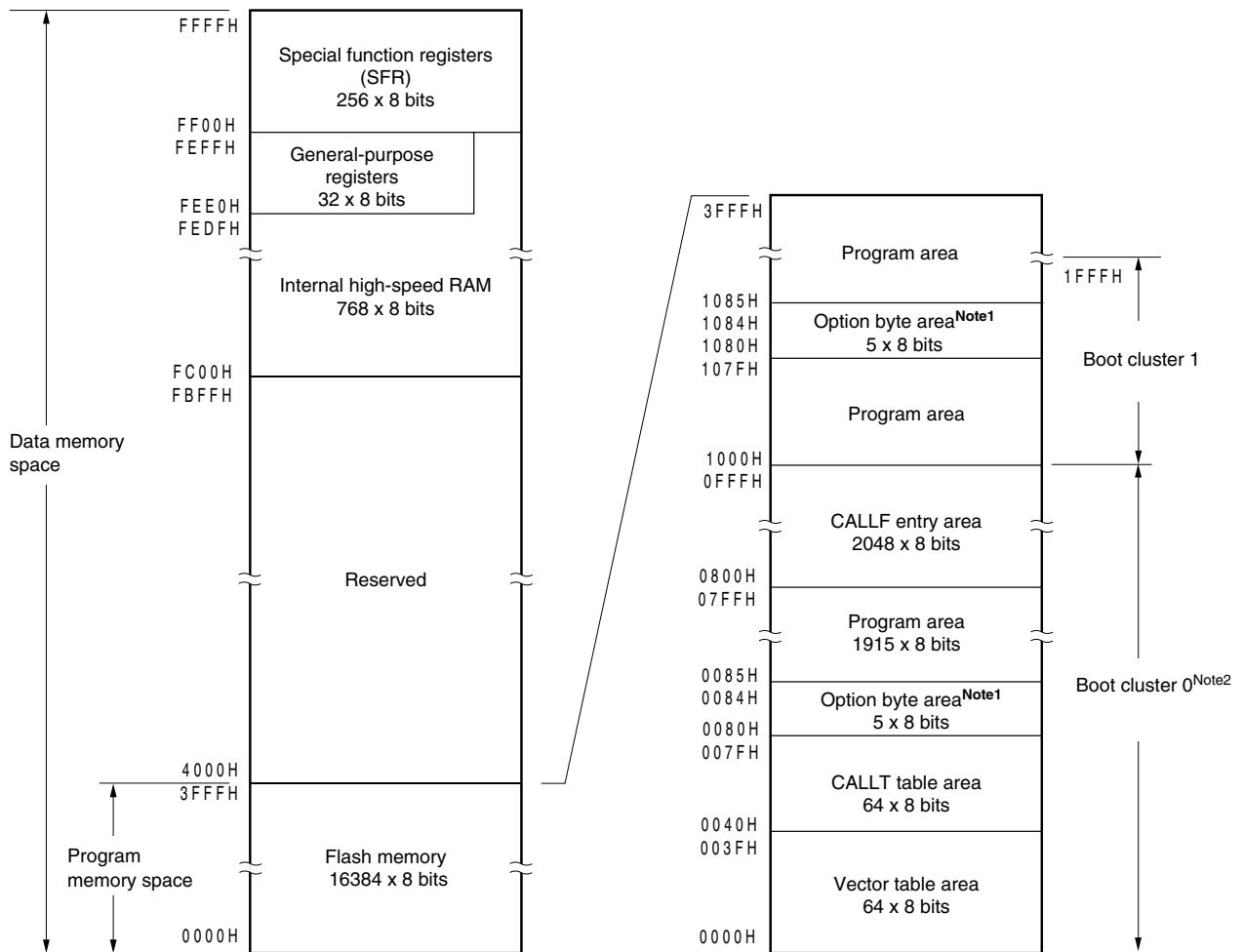
Figure 3-1. Memory Map ( \mu PD78F0521)
