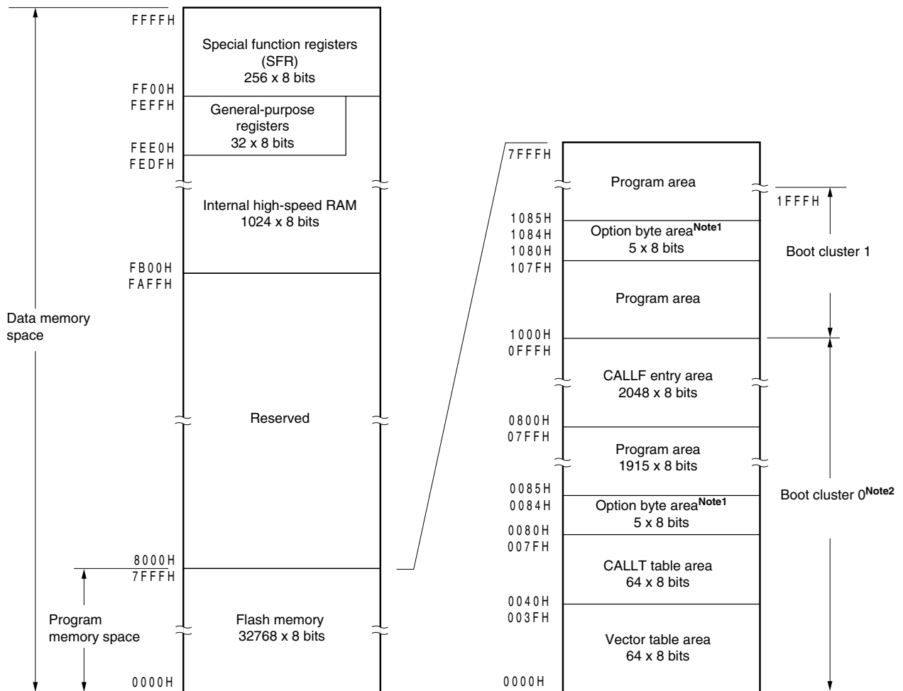
Figure 3-3. Memory Map ( \mu PD78F0523)
