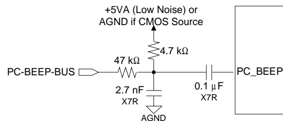
Figure 29. PC_BEEP Input
