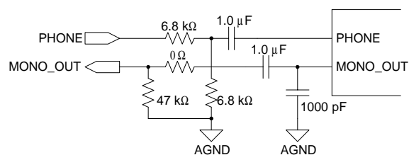
Figure 30. Modem Connection
