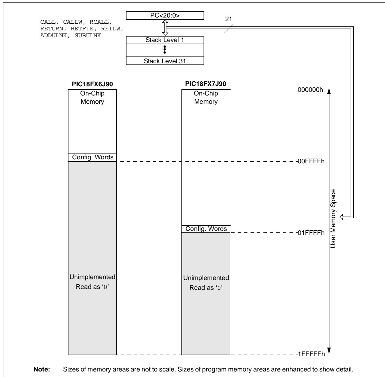
FIGURE 5-1: MEMORY MAPS FOR PIC18F87J90 FAMILY DEVICES
