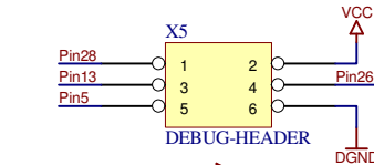
Debug-Header
