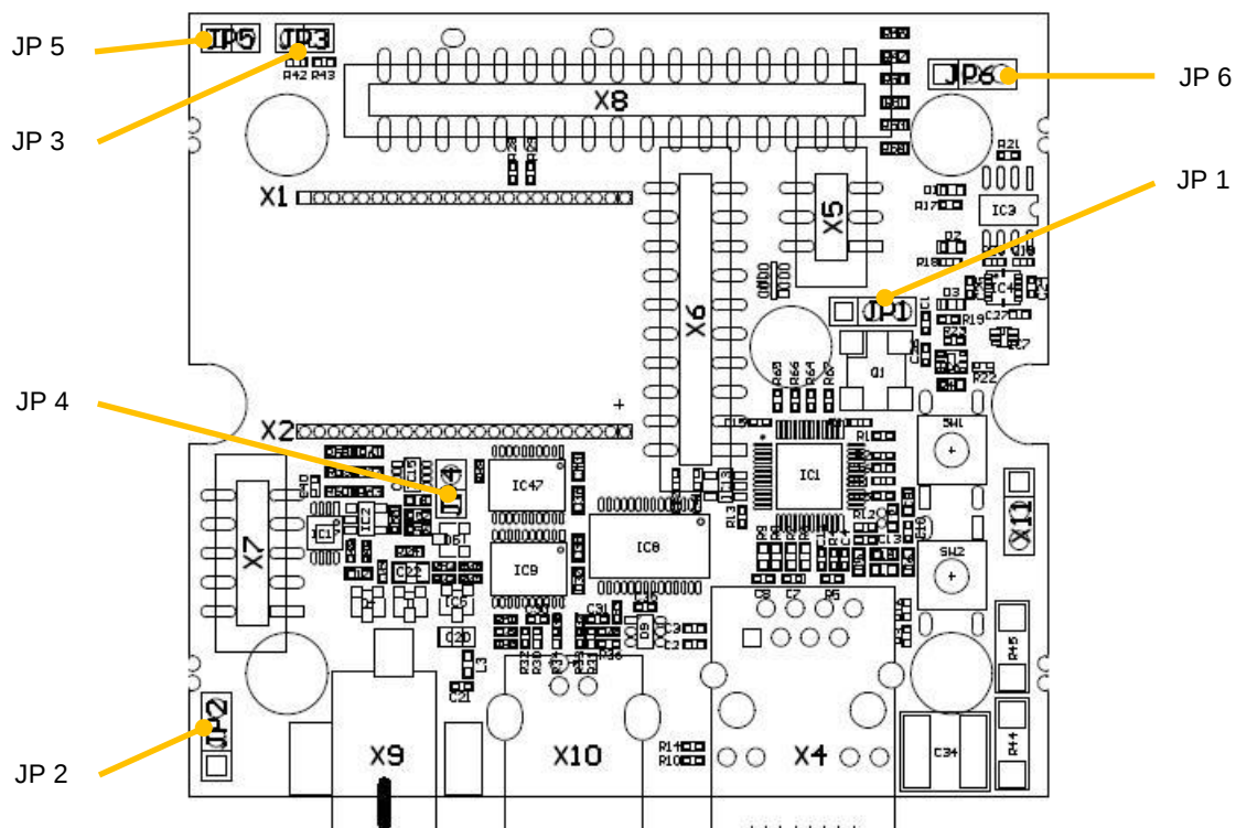
Figure 11: Jumper configuration
