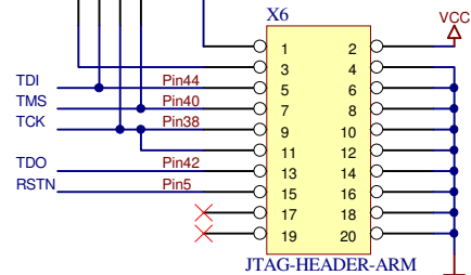
JTAG-Header for ARM
