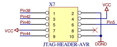
JTAG-Header for AVR
