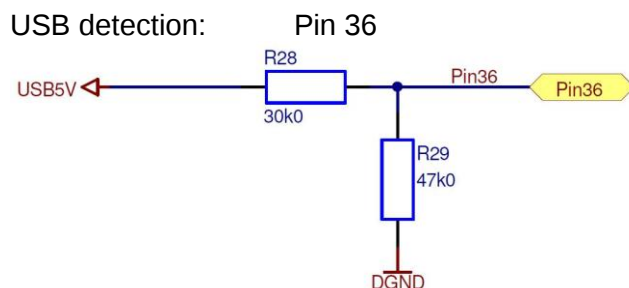
Figure 28: USB supply voltage monitoring
