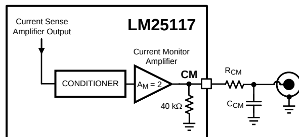
Figure 27. Current Monitor
