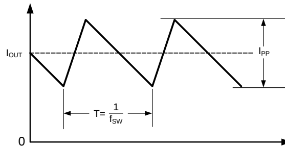
Figure 23. Inductor Current
