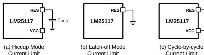
Figure 26. Res Configurations
