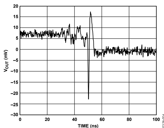
Figure 79. ADV3201 OSD Switching Glitch
