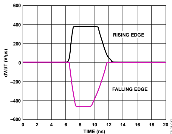
Figure 77. ADV3201 Slew Rate
