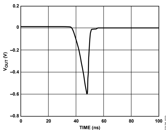
Figure 78. ADV3201 Switching Glitch
