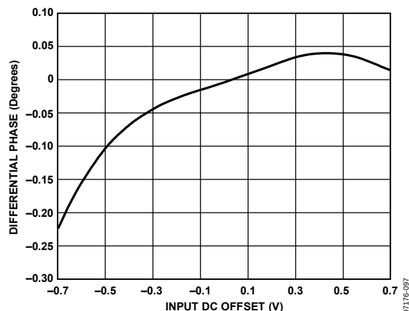
Figure 83. ADV3201 OSD Differential Phase, Carrier Frequency = 3.58 MHz, Subcarrier Amplitude = 300 mV p-p
