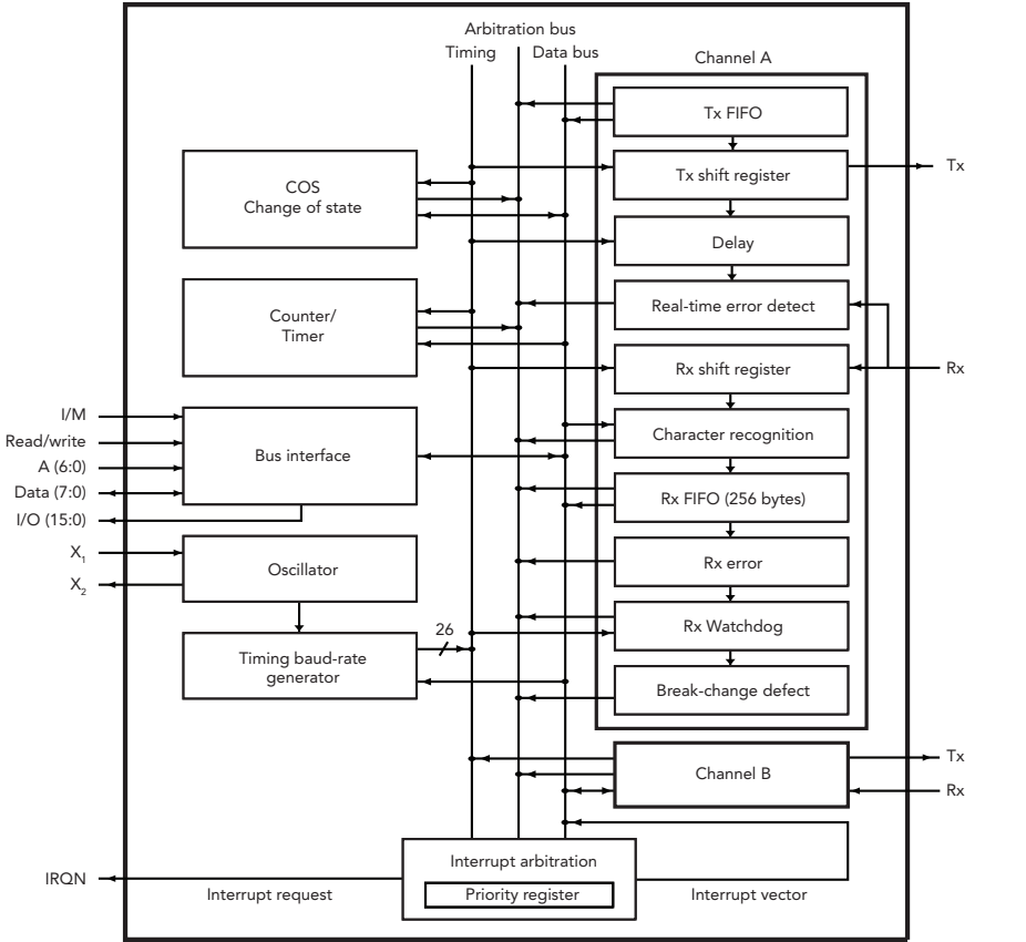
SC28L202 block diagram
