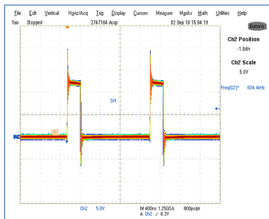
Figure 24 : Inductor node at 25A load Ch2: LX
