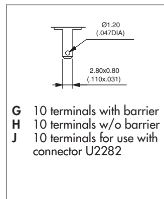
Normalized quick-connect 2,8x0,8
