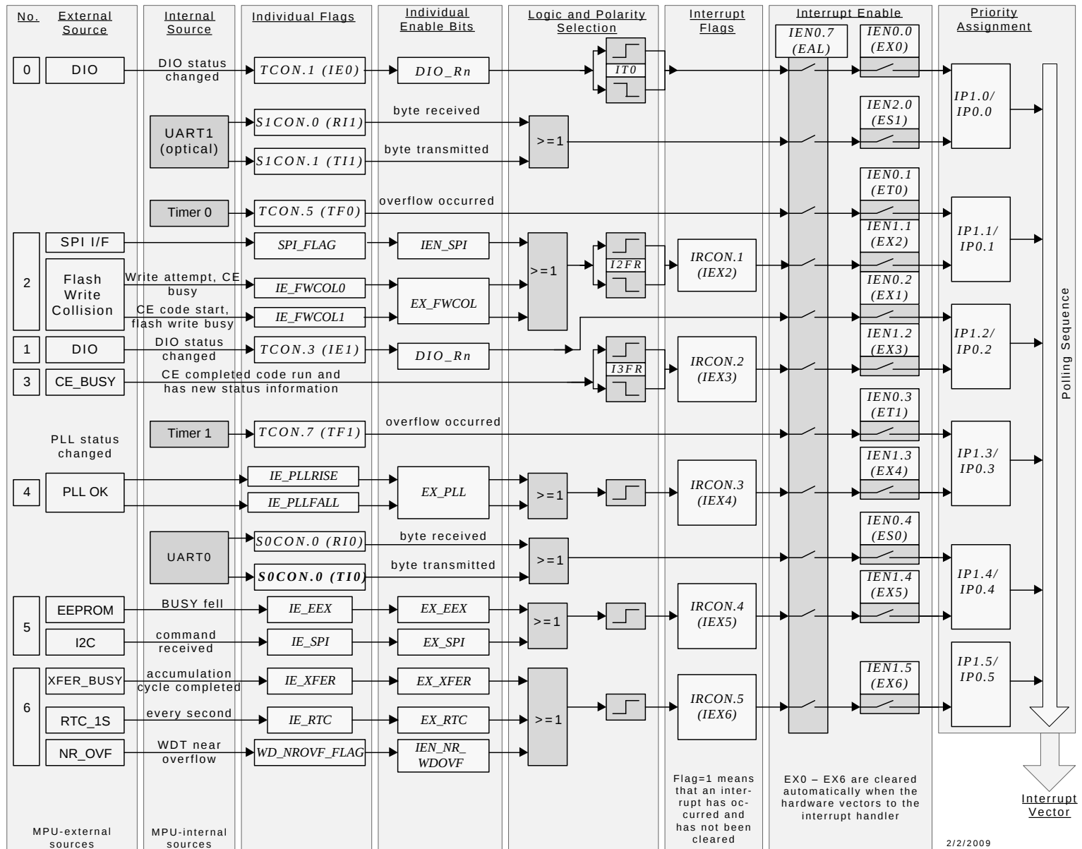
Figure 8: Interrupt Structure
