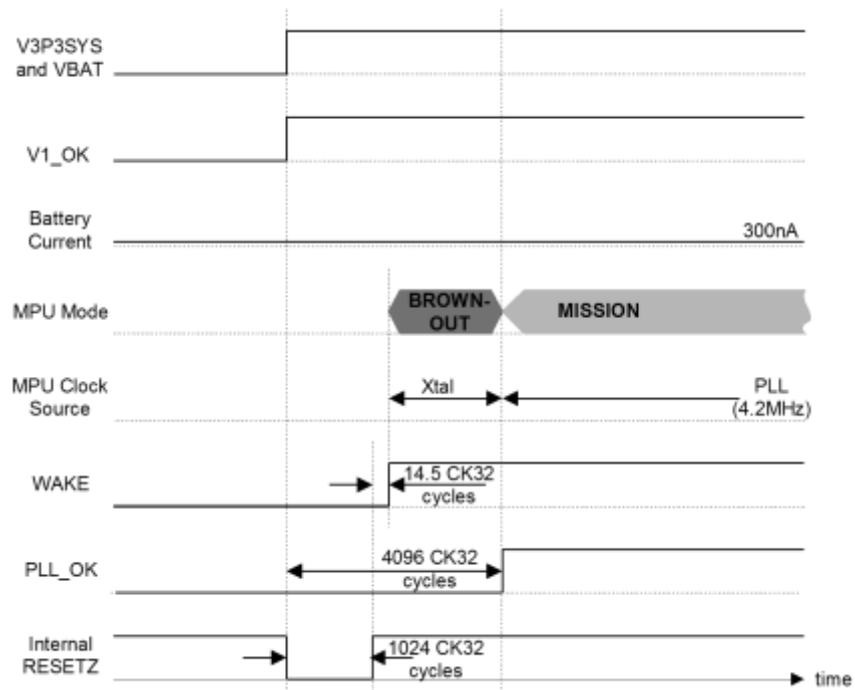
Figure 22: Transition from BROWNOUT to MISSION Mode when System Power Returns
