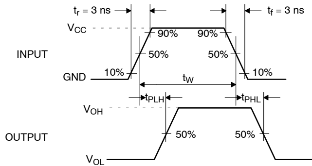
Figure 6. AC Waveforms
