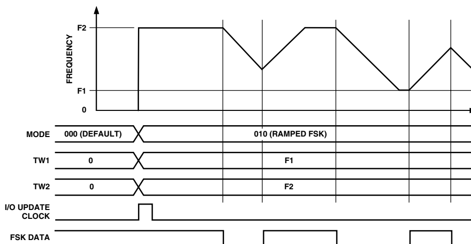
Figure 37. Effect of Premature Ramped FSK Data
