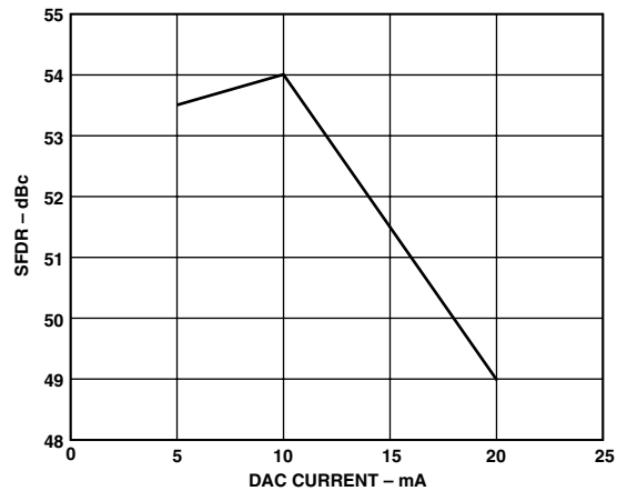
Figure 19. SFDR vs. DAC Current, 59.1 A OUT , 300 MHz REFCLK with REFCLK Multiplier Bypassed
