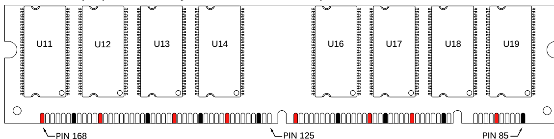
Back View (Populated only for 256MB module)
