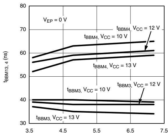
t_{BBM3,4} vs. V_{CC} vs. V_{INDET}
