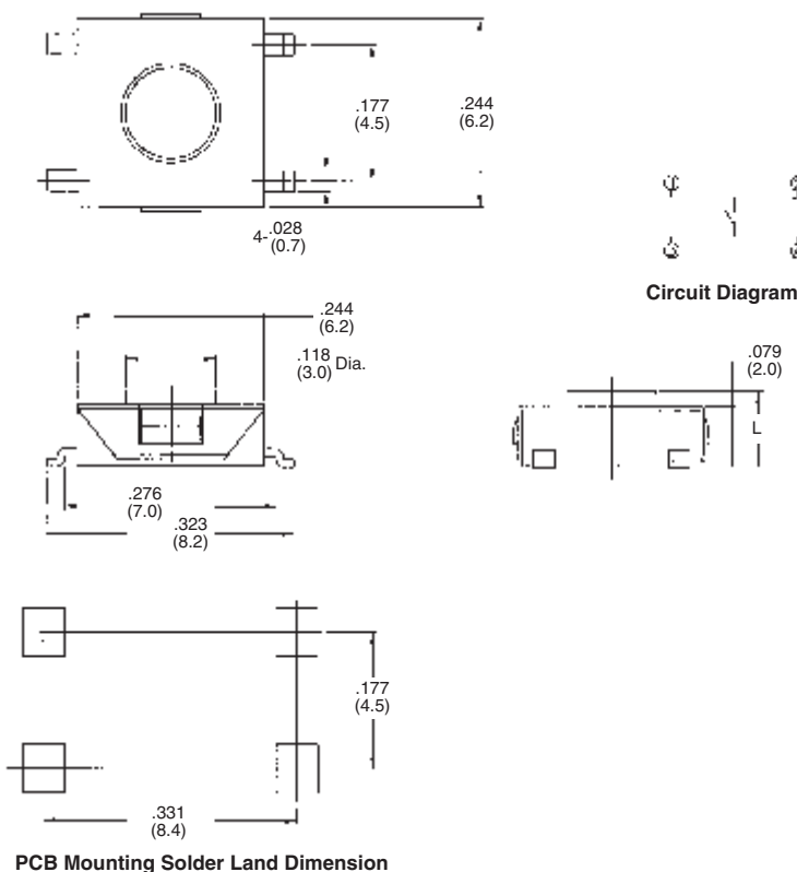
PCB Mounting Solder Land Dimension
