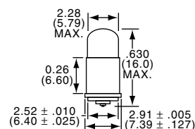
FLANGE BASE- T1 3/4
