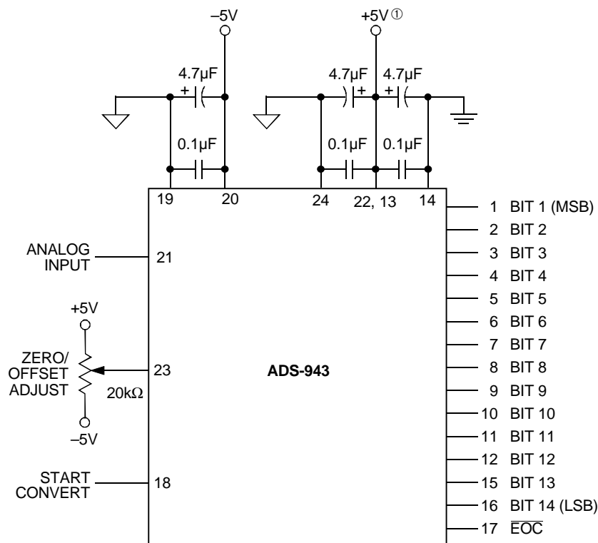
Figure 3. Connection Diagram
