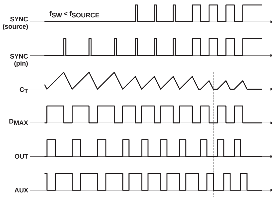
Figure 6. Synchronization Waveforms
