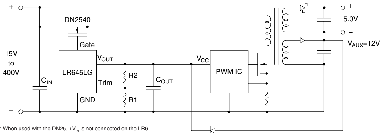
Figure 2: High Current SMPS Start-Up
