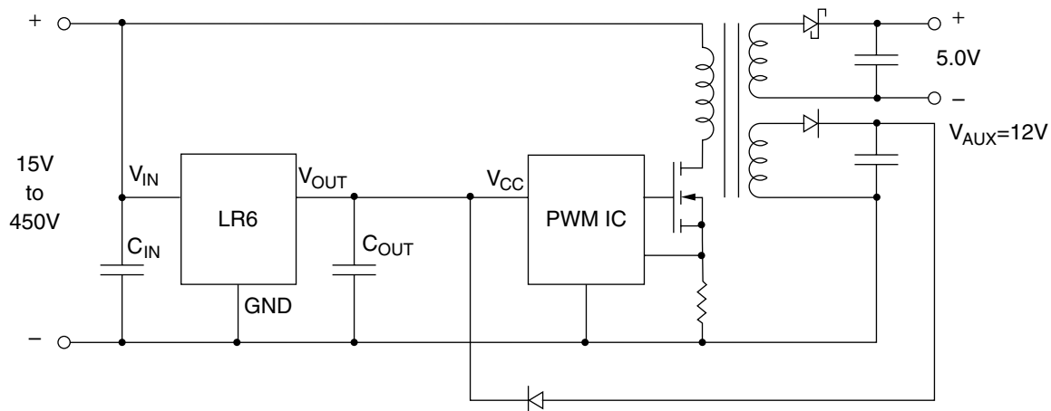
Figure 1: SMPS Start-Up Circuit
