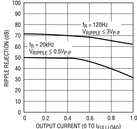
LT1083/4/5-5 Ripple Rejection vs Current
