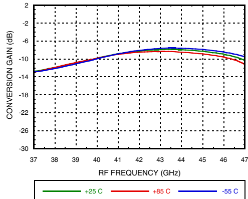
Conversion Loss vs. Temperature
